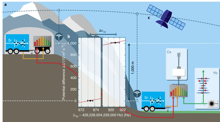
FIGURE 13.3. • Relativistic Geodesy: By now, optical clocks have become small enough so that one can use them to measure heights [248]; this establishes the field of \uparrow relativistic geodesy : the measurement of differences in the gravitational potential by exploiting generally relativistic effects and our technological ability to measure times extremely precisely.
