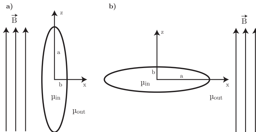
Abbildung 1: Sketches of the two cases a) prolate (cigar shaped) b) oblate (discus shaped) object, within a magnetic field.
